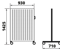
Louvre Trolley dimensions (mm)
